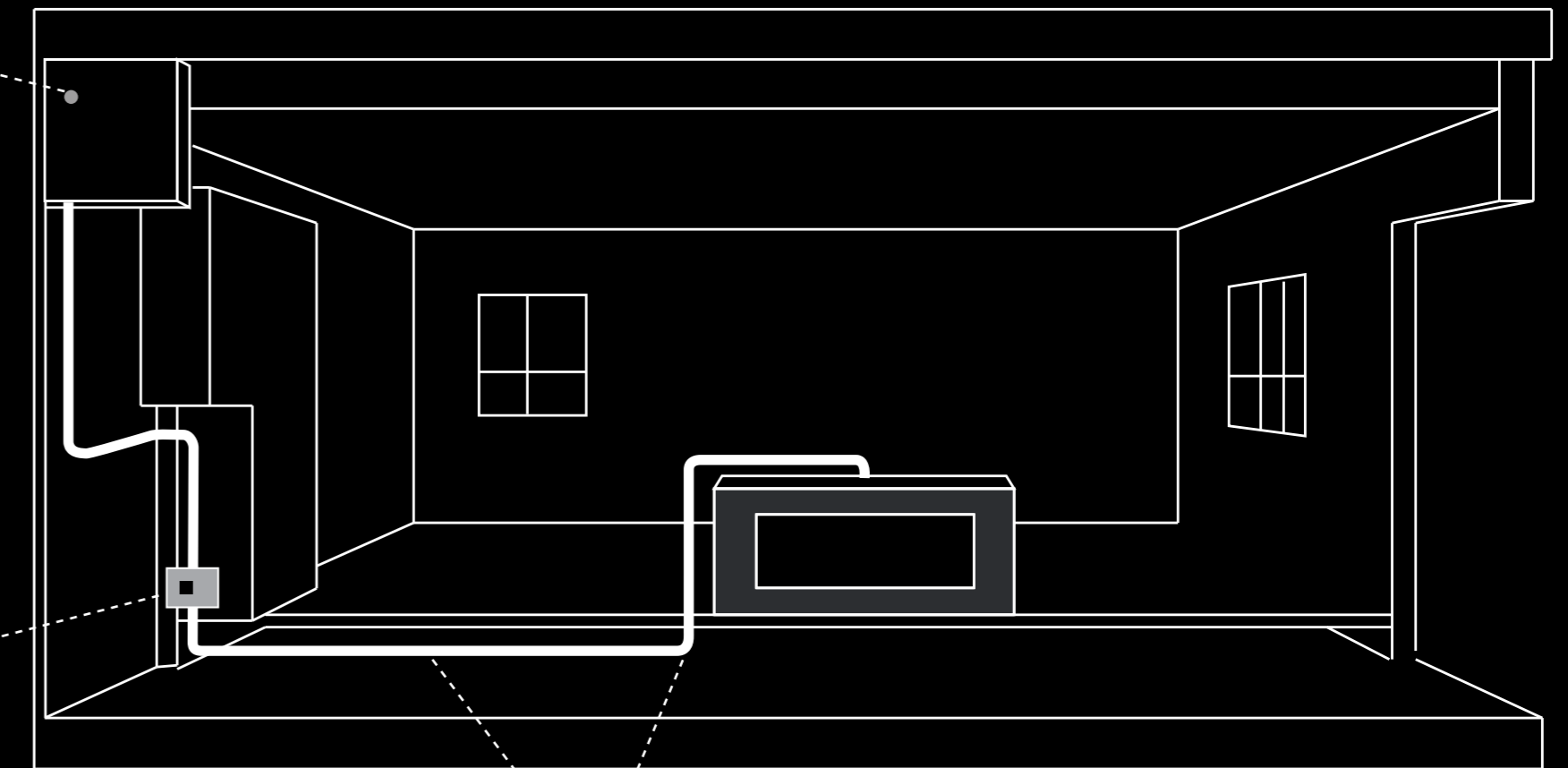
Flush Horizontal End-Line Termination
